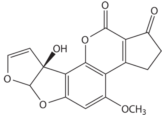
Analyte: Aflatoxin M1 (AFLA M1)
