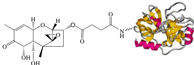
Conjugate of Deoxynivalenol (DON) with Peroxidase (POD)
