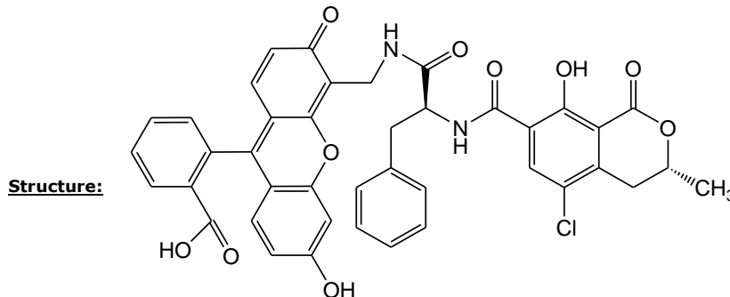
Ochratoxin A (OTA), fluorescein labeled
