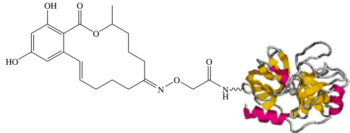
Conjugate of Zearalenone-carboxymethyloxime with Horseradish Peroxidase (HRP)
