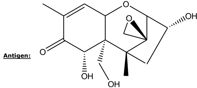
Antigen structure: Deoxynivalenol (DON)
