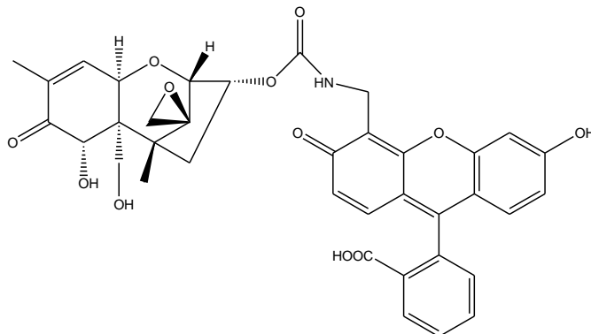
Deoxynivalenol (DON) covalently bound to Fluorescein
