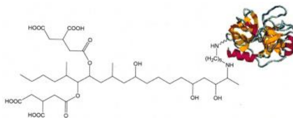
Conjugate of Fumonisin B1 with Ovalbumin (OVA) (FUM-OVA)
