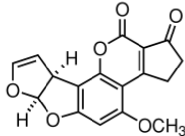
Aflatoxin (AFLA)
