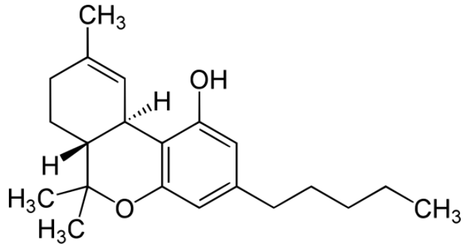
Antigen structure: Tetrahydrocannabinol (THC)
