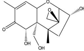
Deoxynivalenol (DON)
